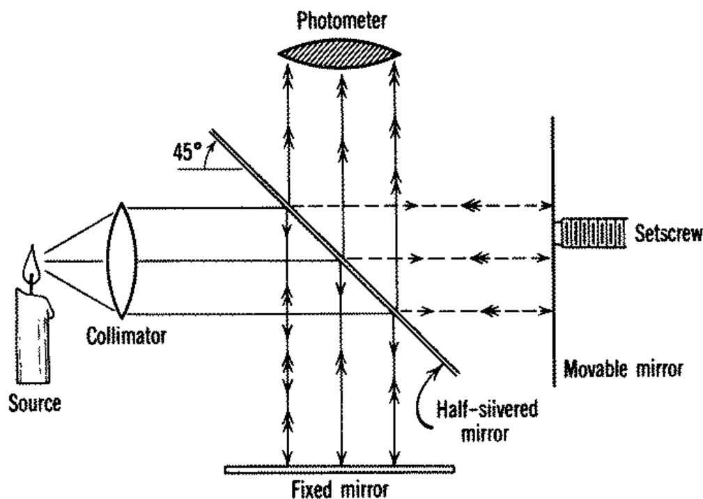
MICHELSON INTERFEROMETER
